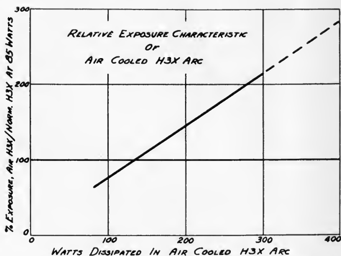
FIG. 4. Exposure of air-cooled H3X arc referred to a normal H3X arc operated at 85 watts.
